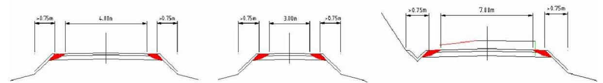
C. Access road to the wind farm. Transportation of components and Internal wind farm road without circulation of cranes (wind farms in the United States)
