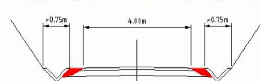
B.- Internal wind farm road with crane movement
