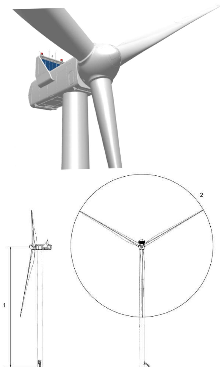
Figure 11-1: Illustration of outer dimensions – structure
