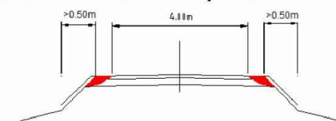
B.- Internal wind farm road with crane movement
