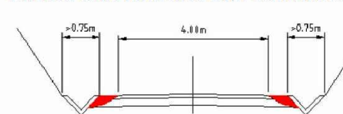
B.- Internal wind farm road with crane movement
